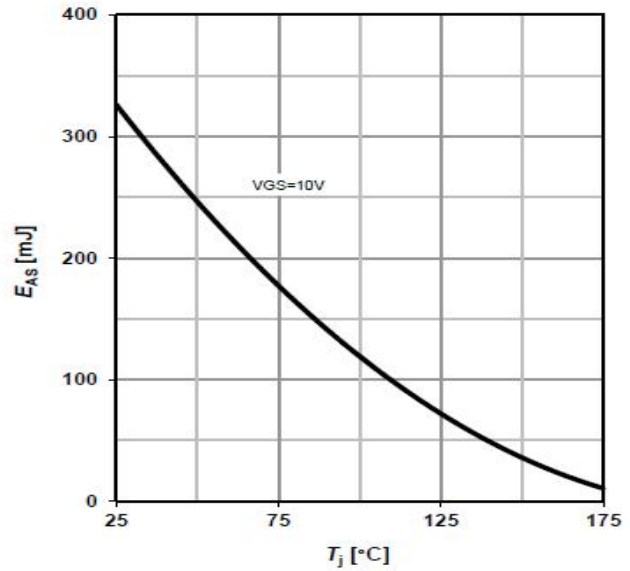
Avalanche energy
