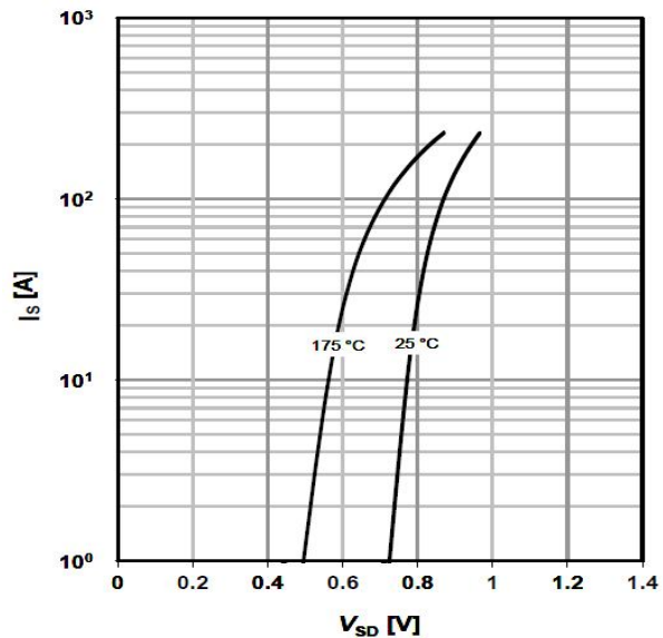
IS -- VSD
