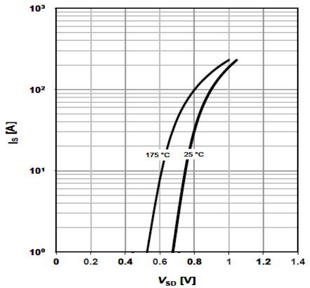
IS -- VSD
