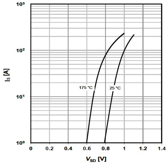
IS -- VSD
