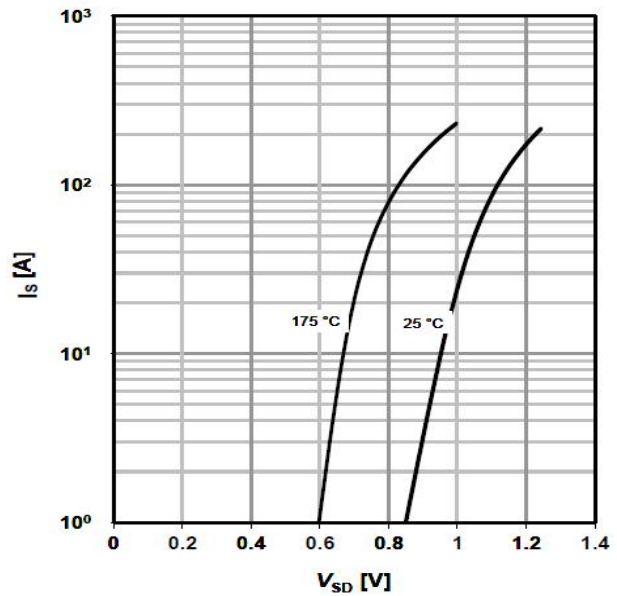
IS -- VSD
