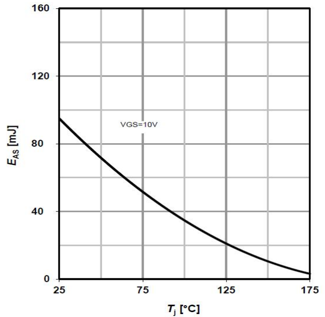
Avalanche energy
